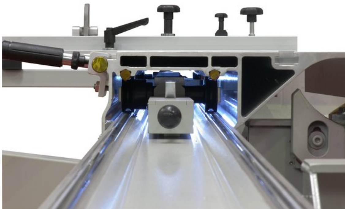
Heavy duty sliding table
